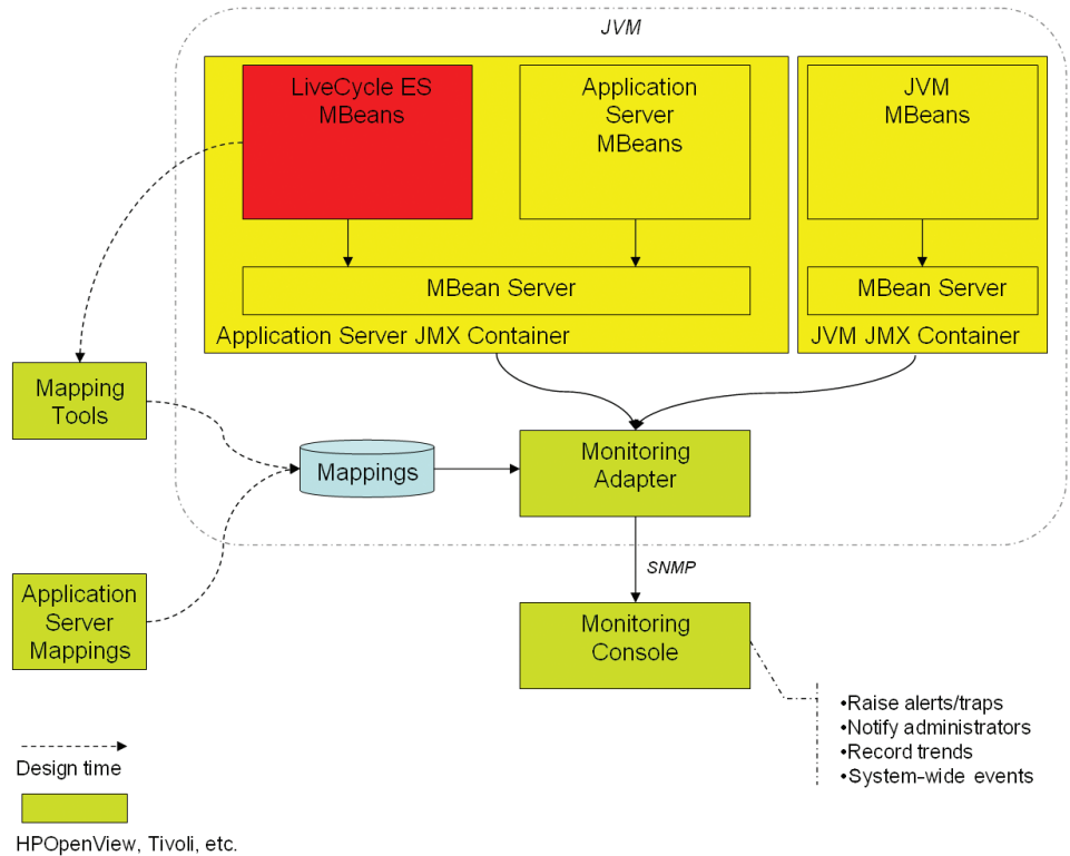
Figure 2. JMX monitoring
