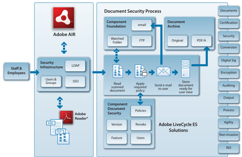
Architecture of a security system built on LiveCycle Rights Management ES software
