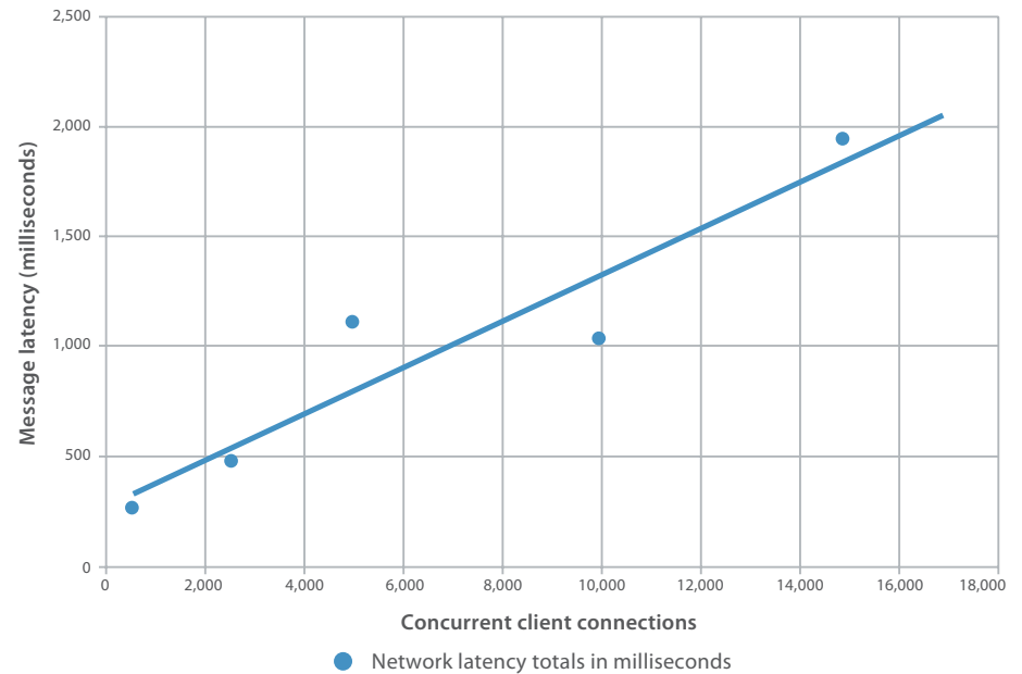
Message latency versus client connection count.
