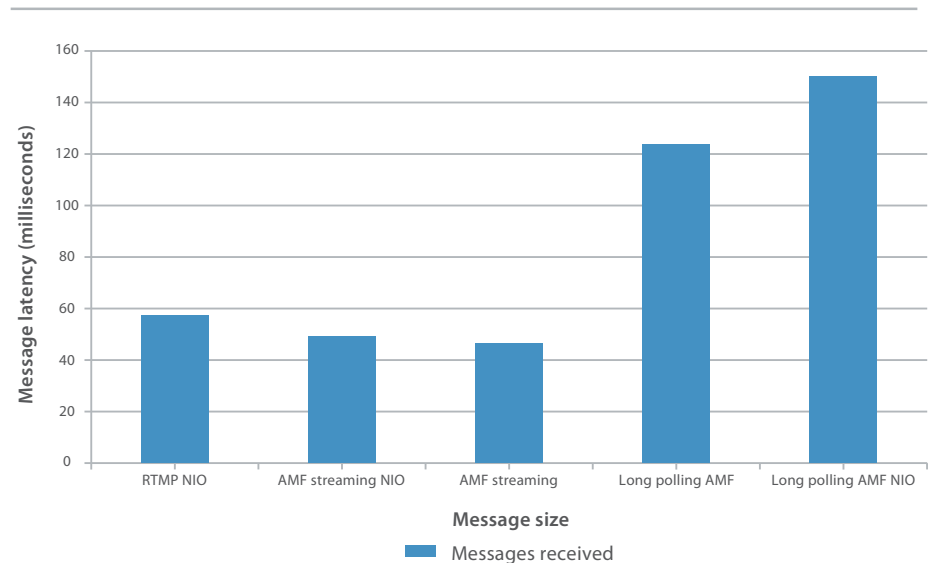
Message latency by channel type
