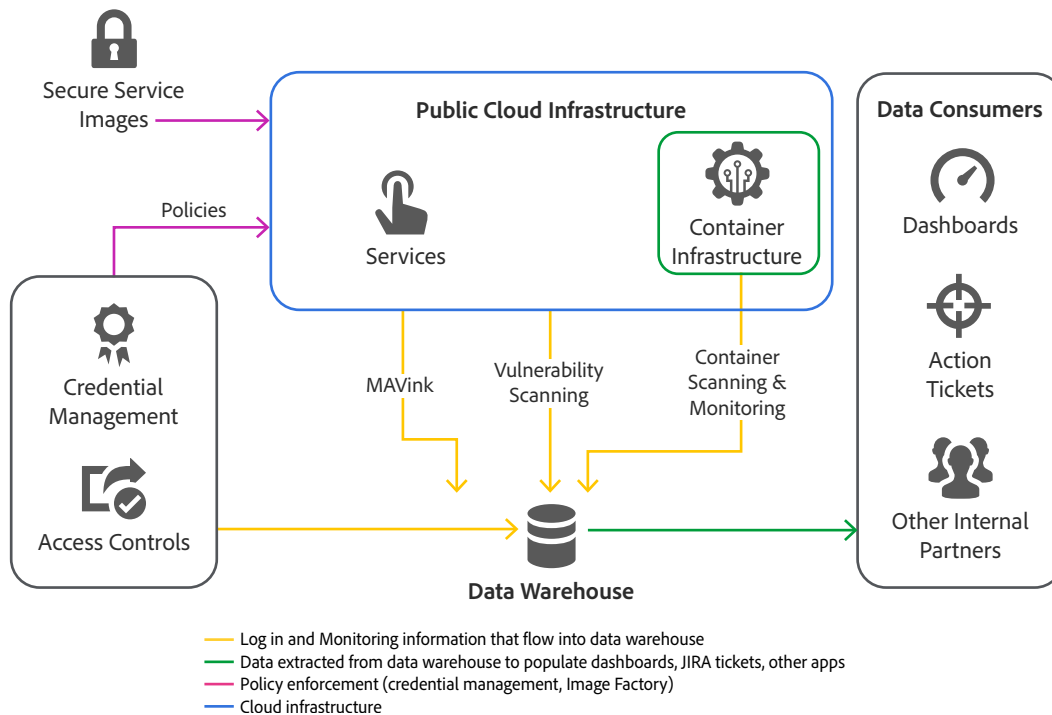
Figure 1: The Adobe OSS Data Flow
